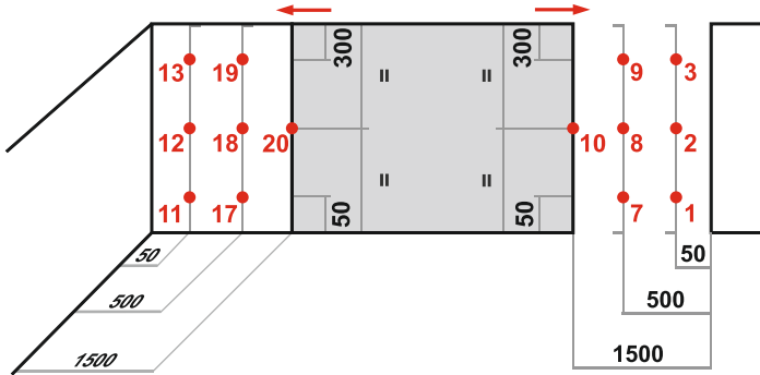
Cancello scorrevole Sliding gate Cancela corredera Schiebetor Porte coulissante
